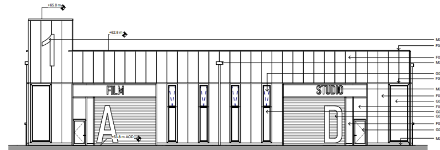
① GW01 - North East Elevation 1 : 100
