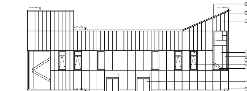
02 Greenhill Works entrance, East elevation
