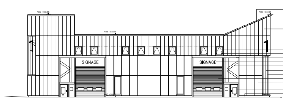
01 Greenhill Crescent, North elevation
